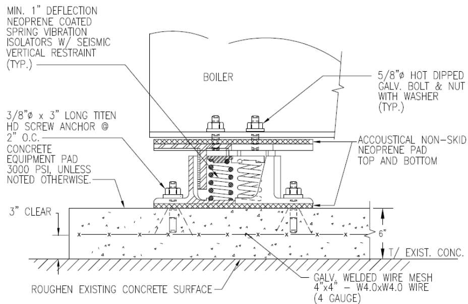
4 BOILER UNIT MOUNTING DETAIL NO SCALE
